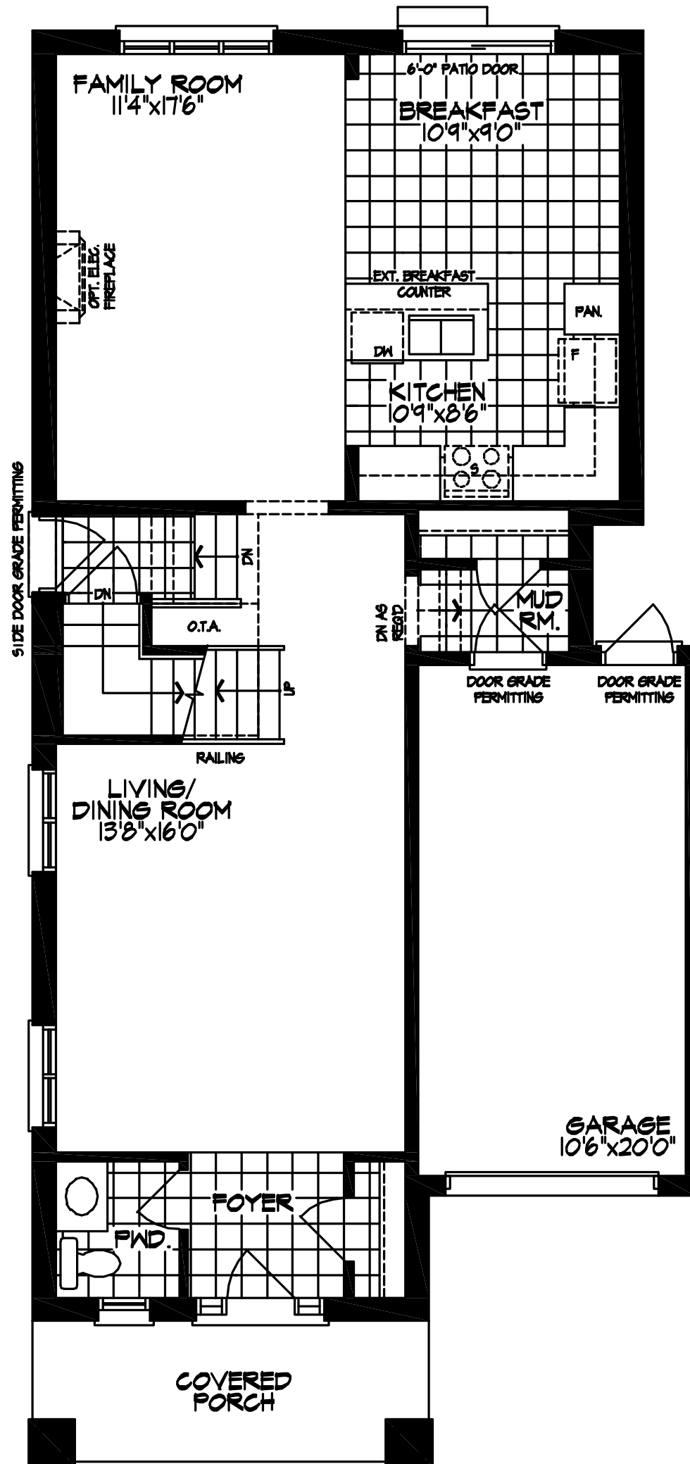
GROUND FLOOR ELEVATION A1 & A2 (REV)
